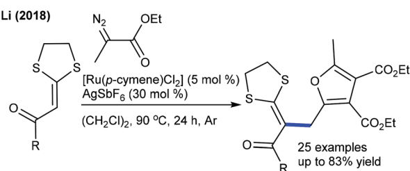
Scheme 41 Furfurylation of \alpha -acylketene dithioacetals with \alpha -diazoketones.
