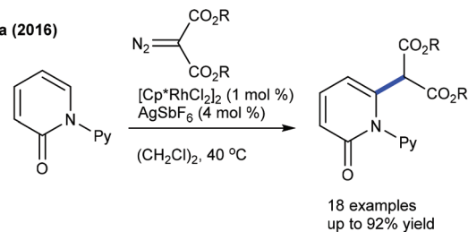
Scheme 49 C6-Alkylation of pyridones using diazo compounds.
