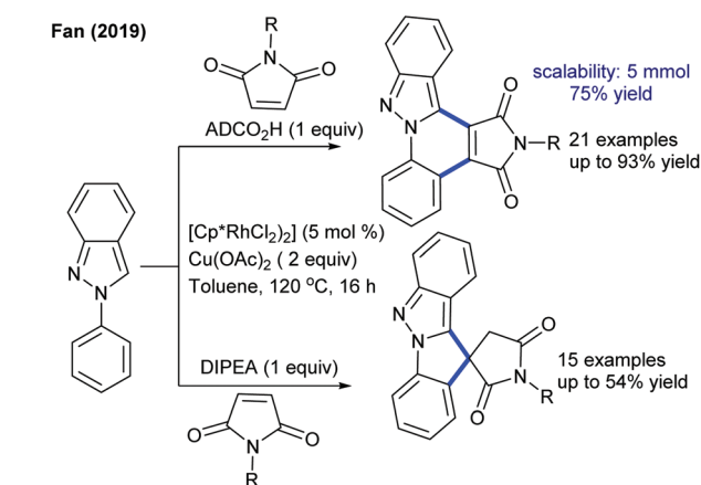
Scheme 89 Oxidative annulation of 2-aryl indazoles with maleimides.
