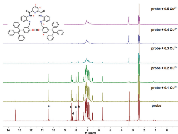
Fig. 6 ^1\text{H} NMR spectroscopic titration spectra of probe@Cu 2+ on increasing concentrations of \text{Cu}^{2+} in d-DMSO solution.
