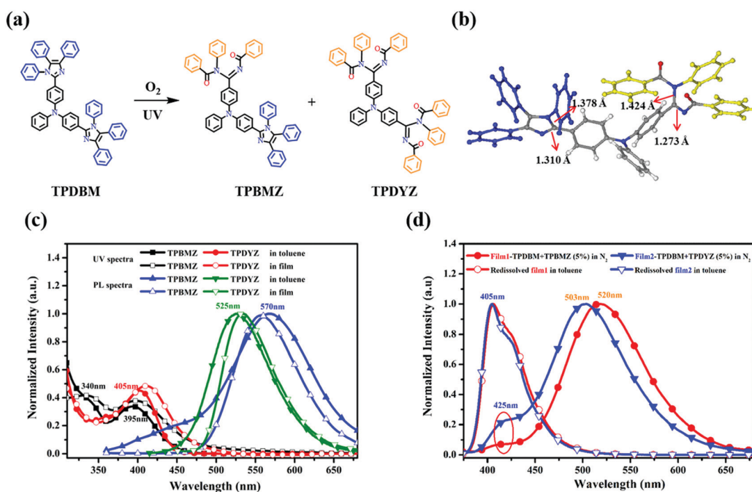
Fig. 5 (a) The photochemical reaction changing the molecular structure from TPDBM to TPBMZ and TPDYZ. (b) The single crystal structure of TPBMZ. (c) The UV and PL spectra of TPBMZ and TPDYZ both in toluene solution and film states. (d) The PL spectra of TPDBM doped with 5% (molarity) TPBMZ and TPDYZ in film form under pure N_2 and in toluene solution under air.
