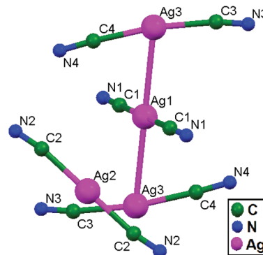
Fig. 5 The compound \text{Ti}[\text{Ag}(\text{CN})_2] , 5 , showing three crystallographically distinct silver atom sites with ligand-unsupported argentophilic interactions.
