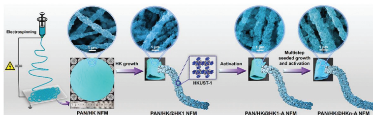
Fig. 11 Schematic illustration of electrospun PAN/HKUST-1 composite fibers used as a skeleton to prepare a self-supported and flexible HKUST-1 nanofibrous membrane (NFM) with ultrahigh HKUST-1 loading and stable and uniform HKUST-1 growth. Reprinted with permission from ref. 140. Copyright 2018 American Chemical Society.
