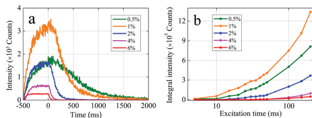
Fig. 3 (a) Rising times and lifetimes of single UCNP particles with different \text{Tm}^{3+} doping concentrations under a power density of 0.48 \text{ MW cm}^{-2} . (b) Trends and total emission intensity integrals of single UCNP particles with different \text{Tm}^{3+} doping concentration changes according to excitation time.
