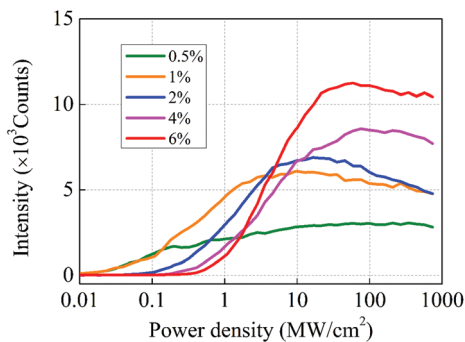
Fig. 2 Measured upconversion luminescence intensities of single UCNP particles with different \text{Tm}^{3+} doping concentrations at different excitation power densities. Here, the intensity is the sum of the emission intensity for wavelengths in the range of 400–842 nm.
