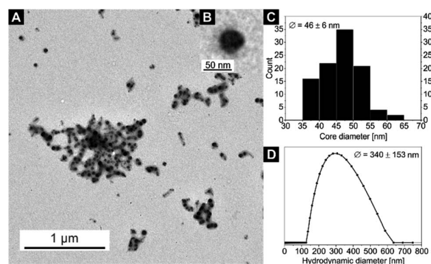
Fig. 5 (A) TEM image of sample 8. (B) An inset with a zoom on a single nanoparticle. (C) Core size distribution D_{\text{core}} (from TEM) and (D) hydrodynamic diameter distribution D_{\text{h}} (from DLS) of sample 8 (for DLS autocorrelation function see Fig. S11†).
