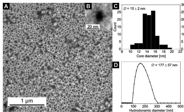
Fig. 4 (A) TEM image of sample 7. (B) An inset with a zoom on a single nanoparticle. (C) Core size distribution D_{\text{core}} (from TEM) and (D) hydrodynamic diameter distribution D_{\text{h}} (from DLS) of nanocomposite sample 7 (for DLS autocorrelation function see Fig. S11†).
