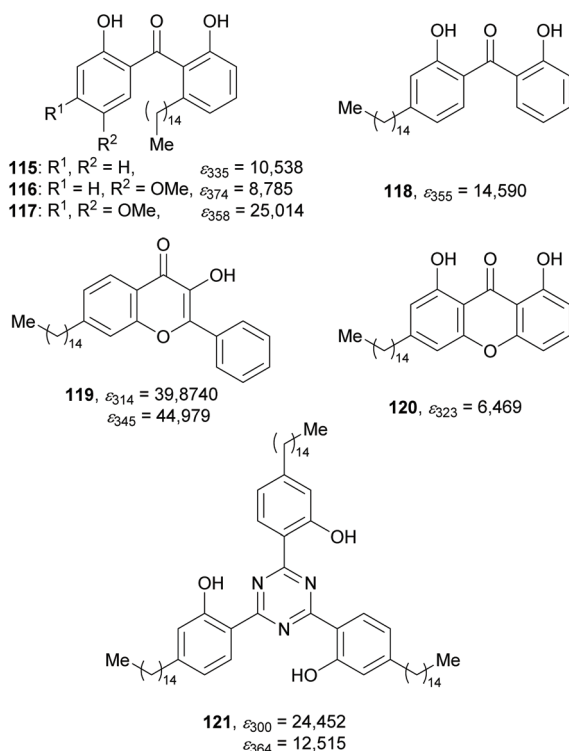
Scheme 12 Examples of the synthesised UV-absorbing compounds by Opatz et al. and their respective \epsilon values (in L\ mol^{-1}\ cm^{-1} ).
