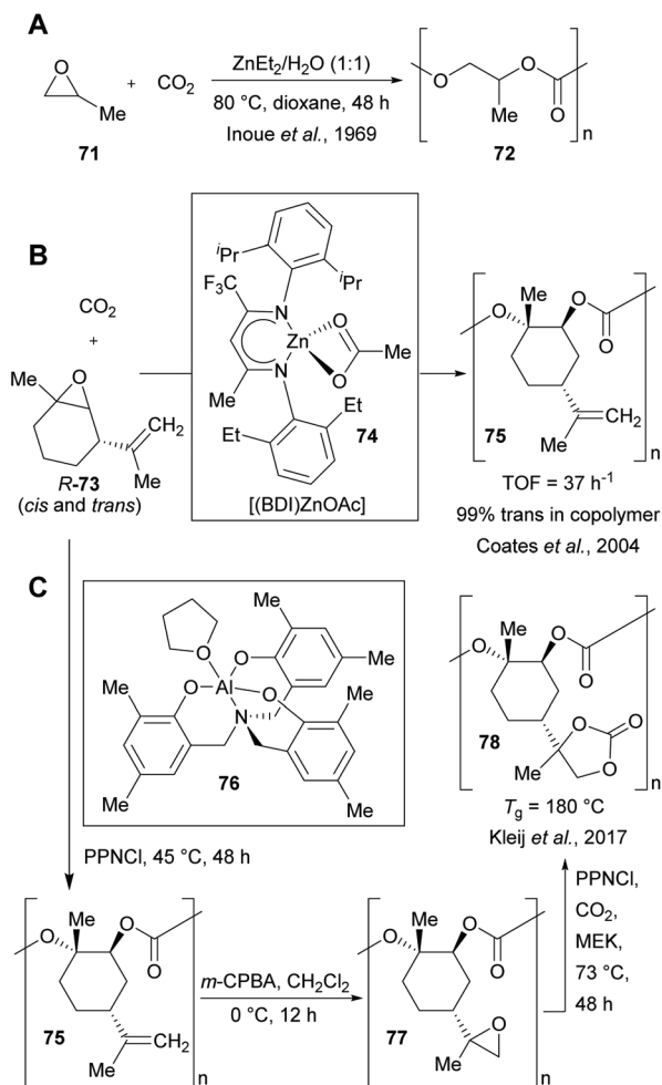
Scheme 7 Copolymerisation of CO 2 with propylene oxide (71, A) or (R)-limonene oxide ((R)-73) (B and C). [(BDI)ZnOAc] (74) = β-diiminate zinc acetate complex, turnover frequency (TOF) = mol 73 (mol Zn) -1 h -1 , PPNCI = (bis-triphenylphosphine iminium chloride).
