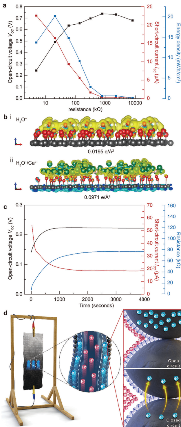
Fig. 4 Effect of resistance and \text{Ca}^{2+} ions on the energy generation of the STEPG. (a) Measured V_{OC} , I_{SC} and energy density values of various resistance STEPGs at 26 °C and 37% RH. (b) Charge redistribution on oxidized graphene covered by hydronium ions (i) and hydronium ions with calcium ions (ii) (yellow, losing an electron; blue, gaining an electron). The value of the electron redistribution on the carbon is located below each panel. (c) Measured V_{OC} , I_{SC} and resistance profiles after stabilization for 3 hours to reduce the water content and resistance change. (d) Schematic illustration of dielectric scattering on the working STEPG and equivalent electric circuit. Blue balls containing arrows represent water molecules along with their polarity (dielectric field) in the inset.
