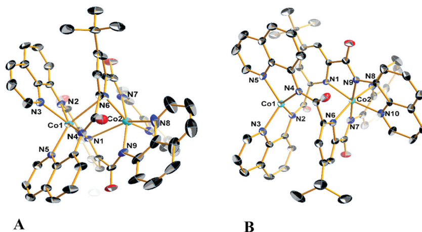
Fig. 3 Molecular structures of (A) the neutral complex in crystals of 2, and (B) cation in crystals of 4 \cdot 1.75\text{CH}_2\text{Cl}_2 with the atom numbering scheme. Displacement ellipsoids are drawn at 50% probability level. Hydrogen atoms have been omitted for clarity. Color code: Co, cyan; C, black; N, blue; O, red.
