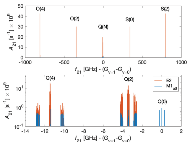
Fig. 10 Einstein A coefficients of E2 (red lines) and M1_{as} (blue lines) transitions of the O(N = 2, 4) , Q(N = 0, 2, 4) and S(N = 0, 2) branches of the fundamental vibrational transition |\nu = 0, N\rangle \rightarrow |\nu' = 1, N'\rangle . The magnetic field was assumed to be 5 G. The lower panel shows a magnification of the spectrum in the region of the Q branch.
