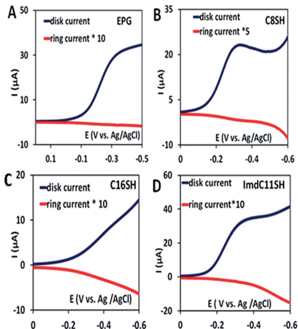
Fig. 4 RRDE data of the complex on the EPG electrode (A), C_8SH SAM modified Au electrode (B), C_{16}SH SAM modified Au electrode (C), and ImdC_{11}SH SAM modified Au electrode (D) at a scan rate of 10 \text{ mV s}^{-1} at 300 rpm using a Pt counter electrode and Ag/AgCl (sat. KCl) as a reference electrode.
