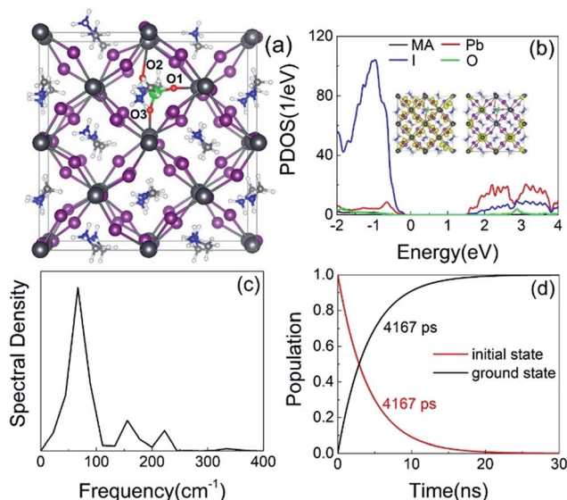
Fig. 6 (a) Optimized IO 3 − geometry. The interstitial iodine and oxygen atoms are colored green and red. (b) PDOS and charge densities of CBM and VBM. (c) Spectral density obtained from Fourier transforms of the autocorrelation functions for the energy gap fluctuation. (d) Evolution of populations of the key states in IO 3 − .
