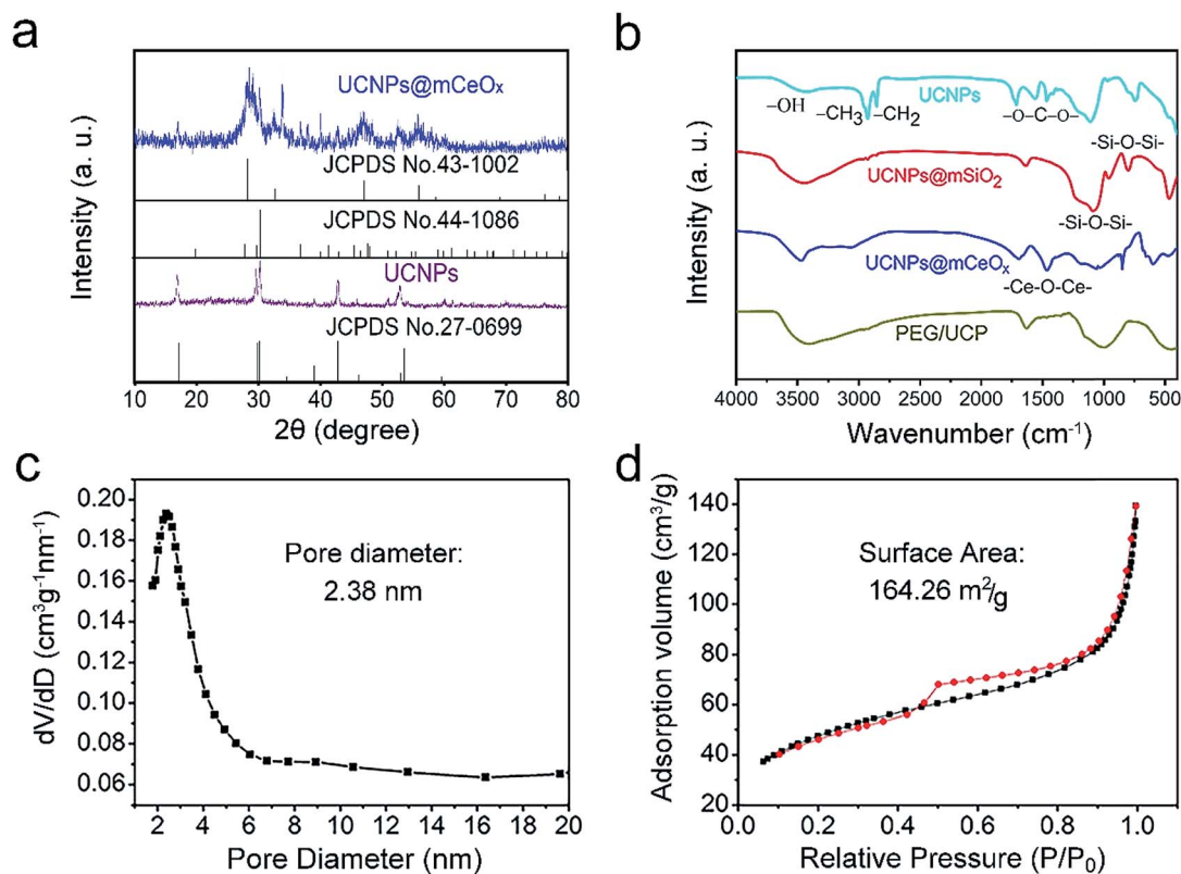
Fig. 2 XRD patterns of UCNP@mCeO x (the standard lines of β-NaGdF 4 , CeO 2 and Ce 2 O 3 are supplied for comparison) (a) and FT-IR spectra of OA-UCNPs, UCNP@mSiO 2 , UCNP@mCeO x and PEG/UCP (b). The pore-size distribution (c) and N 2 adsorption/desorption isotherm (d) of UCNP@mCeO x .
