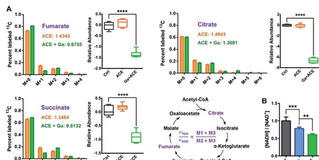
Fig. 5 Combined Ga(III) and acetate treatment leads to reduced TCA cycle flow. (A) Mass isotopomer distributions of 13 C 2 -labelled acetate detected in the TCA cycle and the relative abundances of cycle metabolites. (B) Ratios of bacterial cellular NADH and NAD + levels after treatment with Ga(III) and acetate. Data are presented as mean ± SEM from biological replicates. The asterisks indicate significant difference from the Ctrl or Ga(III) treatment group (**, 0.001 < p < 0.01 and ***, p < 0.001).
