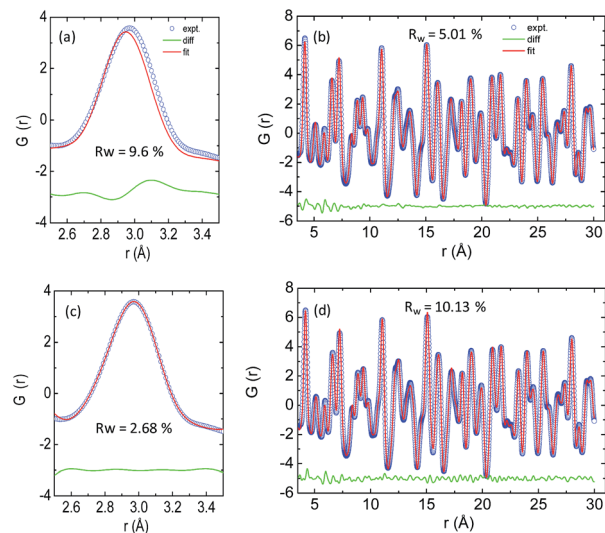
Fig. 6 X-ray PDF data: (a) first peak and (b) total peak fitting using the cubic model. (c) First peak and (d) total peak fitting using the locally distorted model. The experimental data used at a temperature of 100 K.
