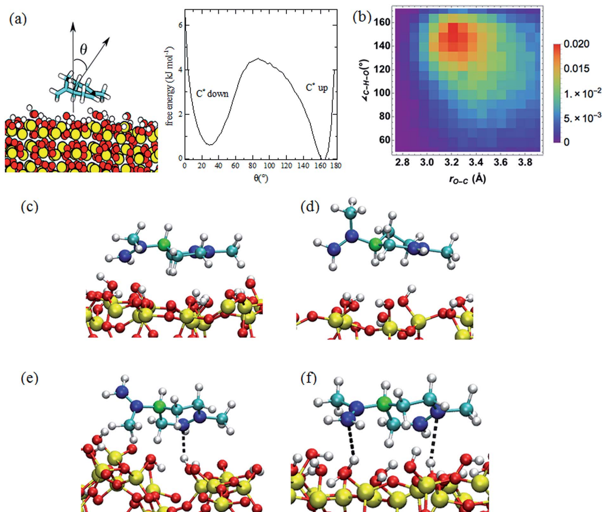
Fig. 2 (a) Limonene reorientation free energy profile on the SiO 2 surface computed from a 0.5 \mu s MD simulation. (b) Probability distribution of the O–C sp 2 distance and C * H–O angle for the nearest hydrogen atoms of SiO 2 to the sp 2 carbon atoms. The probabilities are computed by dividing the count on each bin by the number of steps in the trajectory. (c and d) Snapshots of the limonene molecule in the C * up (c) and C * down (d) orientations. The chiral carbon atoms are colored green, the sp 2 carbon atoms blue, the sp 3 atoms cyan, the silicon atoms yellow, the oxygen atoms red, and the hydrogen atoms white. (e and f) Snapshots of structures corresponding to the one (e) and two (f) hydrogen-bonding interactions between the limonene and SiO 2 surface. The dashed line depicts the hydrogen-bonding interaction.
