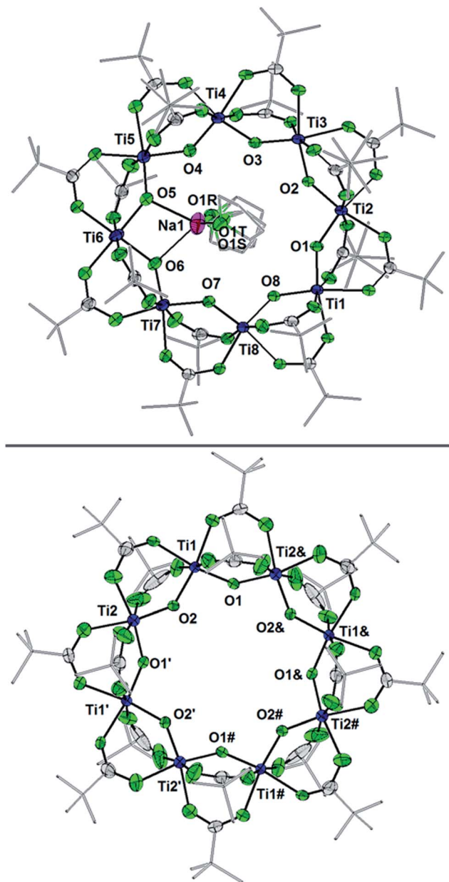
Fig. 6 Displacement ellipsoid (50%) representation of (top) 2-Na and (b) the anion of 2-CoCp 2 * . For clarity, H-atoms are omitted and t Bu groups are shown as sticks. There are two THF ligands to Na + that are disordered, as shown (S: 24.5%, R: 75.5%); see the ESI†. Select bond distances (Å) for 2-Na : Ti1–O8 1.7796(25), Ti1–O1 1.8090(24), Ti2–O1 1.8090(25), Ti2–O2 1.7939(24), Ti3–O2 1.8285(24), Ti3–O3 1.7660(25), Ti4–O3 1.8634(25), Ti4–O4 1.7456(27), Ti5–O4 1.9075(26), Ti5–O5 1.7451(28), Ti6–O5 1.9473(27), Ti6–O6 1.9556(26), Ti7–O6 1.7346(27), Ti7–O7 1.8830(26), Ti8–O7 1.7571(25), Ti8–O8 1.8459(25). Select bond distances (Å) for 2-CoCp 2 * : Ti1–O2 1.8445(1), Ti1–O1 1.7990(1), Ti2–O1' 1.8514(1), Ti2–O2 1.7666(1).
