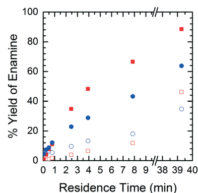
Fig. 9 Product yield as a function of residence time – CFD simulated data (■), experimental data (●), solid symbols = runs at 40 °C, open symbols = runs at 10 °C.
