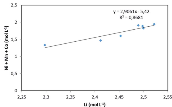
Fig. 6 Stoichiometry between the sum of Ni, Mn, Co concentration and Li concentration in leachate at S/L = 120 \text{ g L}^{-1} during NMC 811 dissolution in 4 \text{ mol L}^{-1} HCl at 25 \text{ }^\circ\text{C} .
