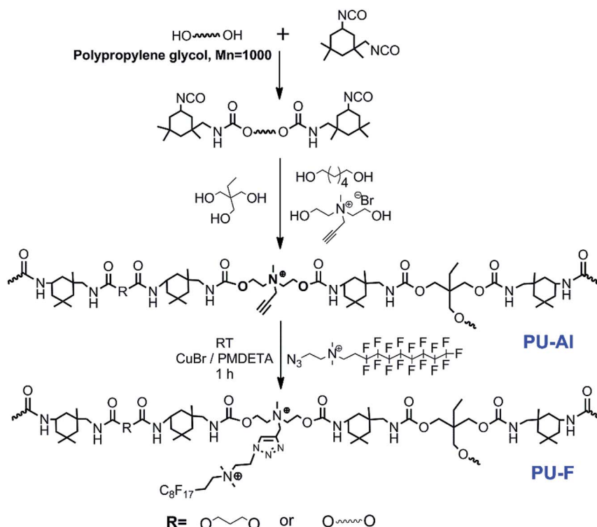
Fig. 3 Two synthetic strategies for the polymers. The synthesis of fluorine-containing polyurethane (PU-F) involved the reaction of PU-Al with compound M3 via click chemistry. The FT-IR spectra provided the evidence of the successful synthesis of PU-F. Fig. 5 shows the successful transformation of PU-Al into PU-F4 by monitoring the disappearance of an azide peak at 2104\text{ cm}^{-1} after click reaction. The PU-F 3 was determined by GPC analysis. The number average molecular weights ( M_n ) and the polydispersity indexes (PDI) of the PU-F 3 was 1.019 \times 10^4\text{ g mol}^{-1} and 1.786, respectively.
