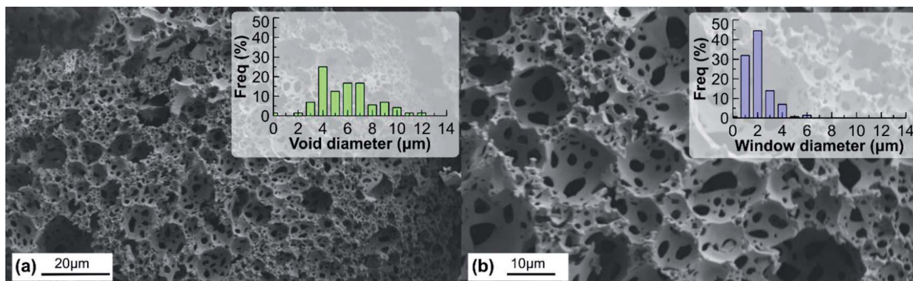
Fig. 1 SEM images of the polyHIPE obtained along with (a) void and (b) window diameter distributions.
