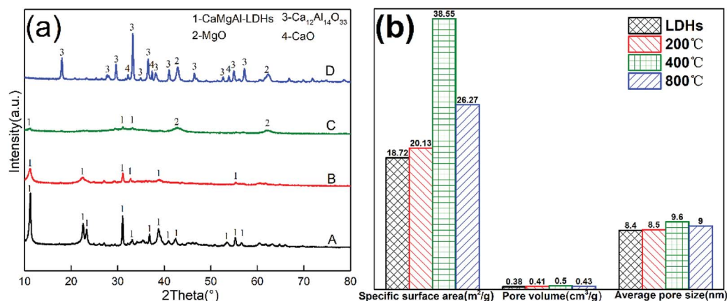
Fig. 5 (a) X-ray diffraction patterns of LDHs calcined at different temperatures for 4 h: (A) as-synthesized, (B) 200 °C, (C) 400 °C and (D) 800 °C (b) BET results of LDHs calcined at different temperatures.
