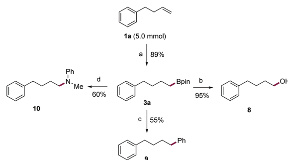
Scheme 2 Gram-scale reaction and transformation of 3a. a 1a (5.0 mmol, 0.66 g), nBuLi (5.0 mol%), HBpin (1.2 equiv.), toluene (5.0 mL), 110 °C, 18 h. b 3a (0.2 mmol), NaBO_3 \cdot H_2O (3.0 equiv.), THF/ H_2O (1/1, 2.0 mL), r.t., 6 h. c 3a (0.2 mmol), bromobenzene (1.5 equiv.), Pd(OAc) 2 (10.0 mol%), rac-BINAP (12.0 mol%), NaOH (15.0 equiv.), THF/ H_2O (5/1, 1.2 mL), 100 °C, 16 h. d 3a (0.2 mmol), N -methylaniline (1.5 equiv.), tBuOOtBu (2.0 equiv.), Cu(OAc)_2 (5.0 mol%), toluene (2.0 mL), 80 °C, 24 h.
