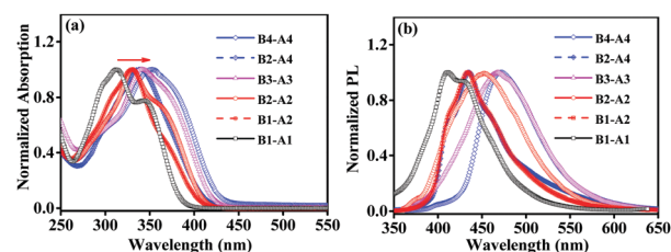
Fig. 2 Normalized absorption (a) and emission (b) spectra of B1-A1, B1-A2, B2-A2, B3-A3, B2-A4 and B4-A4 in THF (concentration: 10 \mu\text{M} ; excitation wavelengths: 344 nm for B1-A1, 329 nm for B1-A2, 335 nm for B2-A2, 340 nm for B3-A3, 338 nm for B2-A4 and 353 nm for B4-A4; EX slit: 5 nm; EM slit: 10 nm).
