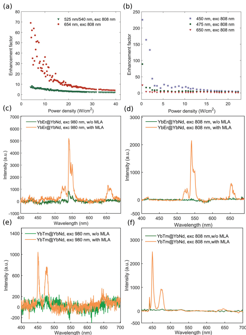
Fig. 3 Excitation intensity dependent enhancement factors induced by the addition of MLA of different emission bands of (a) \text{NaYF}_4\text{:}20\%\text{Yb}^{3+}, 2\%\text{Er}^{3+} @ 20\%\text{Yb}^{3+}, 30\%\text{Nd}^{3+} and (b) \text{NaYF}_4\text{:}20\%\text{Yb}^{3+}, 0.5\%\text{Tm}^{3+} @ 20\%\text{Yb}^{3+}, 30\%\text{Nd}^{3+} nanoparticles under 808 nm CW excitation. UCL spectra of \text{NaYF}_4\text{:}20\%\text{Yb}^{3+}, 2\%\text{Er}^{3+} @ 20\%\text{Yb}^{3+}, 30\%\text{Nd}^{3+} nanoparticles under (c) 980 nm and (d) 808 nm CW excitation with and without MLA light modulation (average excitation intensity: 0.1 \text{ W cm}^{-2} ). UCL spectra of \text{NaYF}_4\text{:}20\%\text{Yb}^{3+}, 0.5\%\text{Tm}^{3+} @ 20\%\text{Yb}^{3+}, 30\%\text{Nd}^{3+} nanoparticles under (e) 980 nm and (f) 808 nm CW excitation with and without MLA light modulation (average excitation intensity: 0.1 \text{ W cm}^{-2} ).
