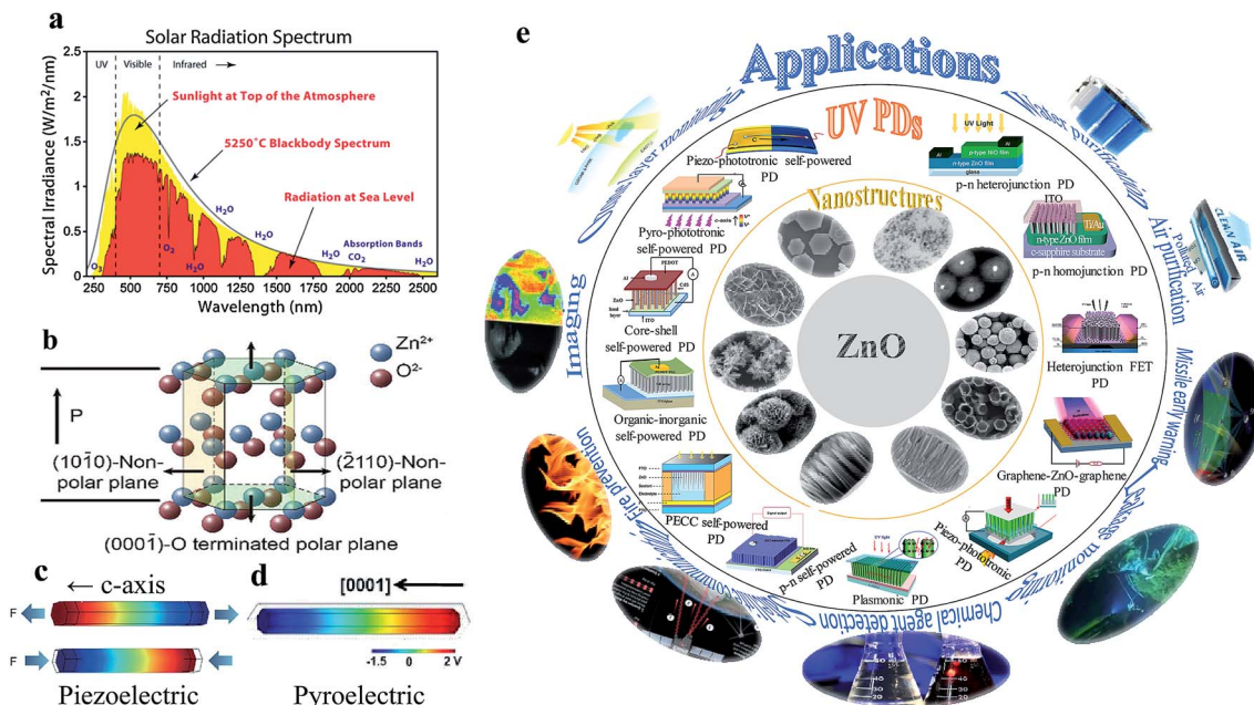
Fig. 1 (a) Total solar radiation spectrum. 12 (b) Atomic model of the ZnO wurtzite structure. Reproduced with permission from ref. 38 Copyright 2019, Wiley-VCH. (c) Simulated piezopotential distribution along a ZnO NW in the presence of strain along the c -axis. Colour gradient indicates the piezopotential generation, where red represents the positive piezopotential and blue the negative piezopotential. Reproduced with permission from ref. 39 Copyright 2009, American Institute of Physics. (d) Electric potential distribution along a ZnO NW when the temperature is decreased from RT 295 to 289 K. Reproduced with permission from ref. 40 Copyright 2012, American Chemical Society. (e) Schematic summarizing the ZnO nanostructures, currently developed UV PDs from conventional to self-powered and their possible future applications.
