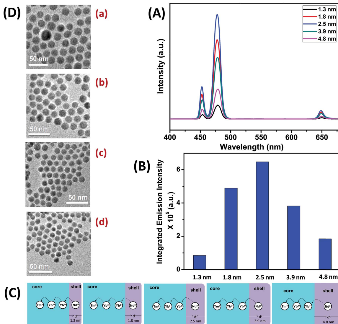
Fig. 3 (A) UCL spectra of CS (30 mol% Nd 3+ ) UCNP shells with different thickness of the NaGdF 4 :Ca 2+ (7)/Nd 3+ (30) shell ( d = 1.3 – 4.8 nm). (B) Integrated intensity of the blue (462–505 nm) emission of CS (30 mol% Nd 3+ ) UCNP shells with different shell thickness ( d = 1.3 – 4.8 nm). (C) Mechanistic investigation of interfacial ET from the Nd 3+ -containing shell to the Tm 3+ containing core in different shell thickness controlled ( d = 1.3 – 4.8 nm) CS (30 mol% Nd 3+ ) UCNP shells. (D) TEM images of CS (30 mol% Nd 3+ ) UCNP shells with different shell thickness ((a) 1.3 nm, (b) 1.8 nm, (c) 3.9 nm and (d) 4.8 nm).
