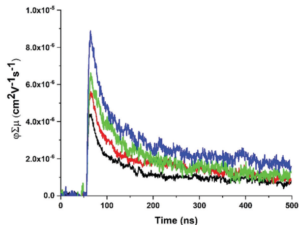
Fig. 5 Representative fp-TRMC transients with increasing fluence ( 1 \times 10^{14} – 4 \times 10^{15} photons per cm 2 ) for a ZnPor-COF-PS film at 700 nm photoexcitation with 7 ns pulse width.
