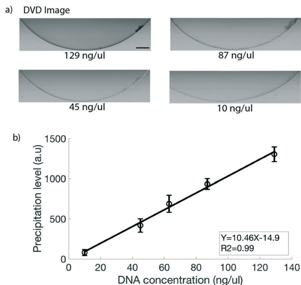
Fig. 5 Lab on DVD generated precipitate images of the known PCR products. a) Calibration images with the lab on DVD platform for concentration ranging from 129 \text{ ng } \mu\text{l}^{-1} to a detection limit of 10 \text{ ng } \mu\text{l}^{-1} . Scale bar: 1 mm. b) Calibration curve of the precipitation level versus known DNA concentration.
