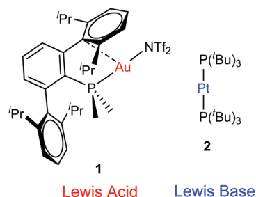
Lewis Acid Lewis Base
