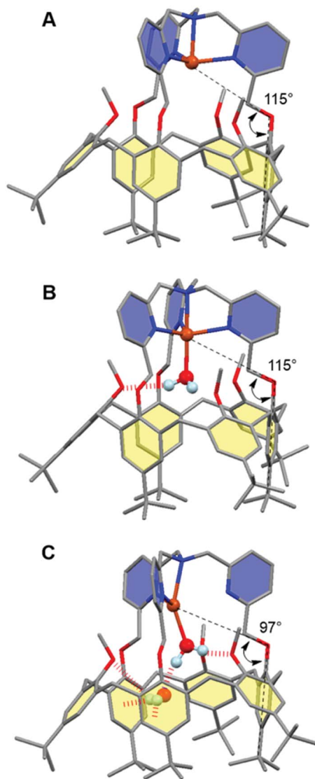
Fig. 7 Representative snapshots extracted from the hybrid DFT/MM MDS for the [\text{Cu}^{\text{II}}/(\text{calix}[6]\text{tmpa})(\text{H}_2\text{O})_x]^{2+/+} complexes (A: \text{Cu}^{\text{I}} , x = 0 ; B: \text{Cu}^{\text{II}} , x = 1 ; C: \text{Cu}^{\text{I}} , x = 2 ). For clarity, solvent molecules (chloroform) and hydrogen atoms are not represented except for the water molecules. The copper ion, the water molecules and the poly-aza cap were treated at the DFT level of theory, and the remaining ones were modelled using Molecular Mechanics. The black dashed lines illustrate the definition of the angles highlighting the partial inclusion of one t Bu group for the [\text{Cu}^{\text{I}}(\text{calix}[6]\text{tmpa})(\text{H}_2\text{O})_x]^+ complexes (Tables S3 and S4†). The red dotted lines indicate hydrogen and OH– \pi bonds. Colour code: grey = carbon, dark blue = nitrogen, red = oxygen, orange = copper, and pale blue = hydrogen.
