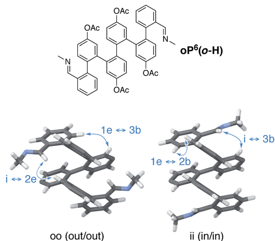
Fig. 9 Optimized geometries of model compound oP 6 (o-H) (PCM(CHCl 3 )/B97-D/TZV(2d,2p)). Acetoxy groups were included in the optimization but are not shown. Key NOESY correlations that were used to make NMR assignments are highlighted.
