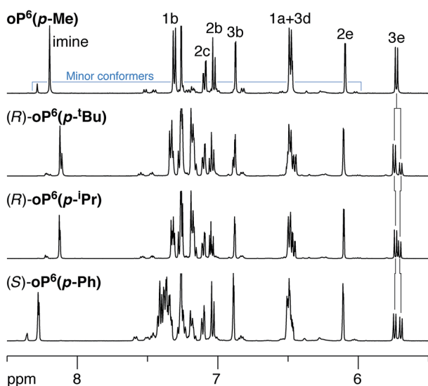
Fig. 3 Representative ^1\text{H} NMR spectra (500 MHz, \text{CDCl}_3 , 273 K) of p -imine o -phenylenes (aromatic region). Protons \text{H}_{3\text{e}} were used to evaluate de's. Small peaks corresponds to misfolded conformers, as confirmed by EXSY spectroscopy.
