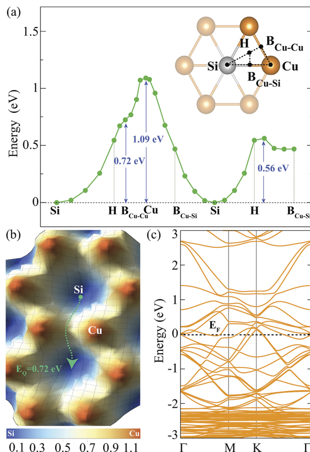
Fig. 2 (a) For a single H adatom, the energy variation between the high symmetry points of the hexagonal structure is demonstrated. The binding energy at Si site is set to zero. (b) Energy landscape for single H adatom adsorbed on Cu 2 Si monolayer. Blue and red colors represent the Si and Cu sites, respectively. E_0 = 0.72\text{ eV} is the lowest energy barrier through the migration path shown with green dashed arrow. The energy values on the scale are in units of eV. (c) Folded electronic band structure of 3 \times 3 \times 1 Cu 2 Si monolayer in which single H adsorbed on Si site. Fermi level, E_F , is set to zero.
