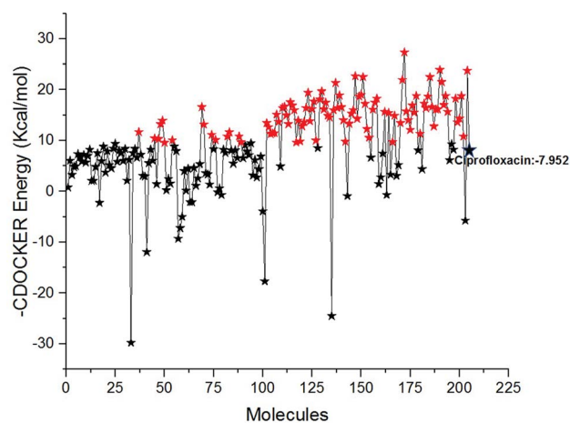
Fig. 6 The–CDOCKER energy score (kcal mol -1 ) of the 204 newly designed FQ analogs. Color code: red stars indicates selected 100 hit compounds having lower–CDOCKER energy ( -9.55 to -29.7924 kcal mol -1 ). Black stars indicated the higher–CDOCKER energy compounds ( -9.47 to +29.7924 kcal mol -1 ).
