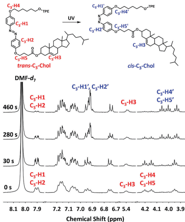
Fig. 6 1 H NMR (400 MHz) of trans -C 3 -Chol gel in DMF- d 7 ( c = 0.45 mM) under UV irradiation at 365 nm ( 0.25 \text{ mW cm}^{-2} ) as a function of irradiation time.
