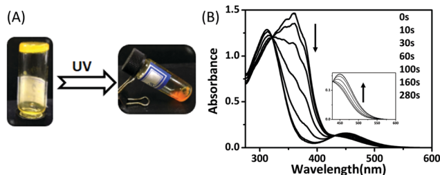
Fig. 5 (A) Photos showing gel-sol transition of trans -C 5 -Chol in DMF ( c = 62 mM) after 15 min of UV irradiation ( 90 \text{ mW cm}^{-2} , 365 nm). (B) UV-Vis spectra of trans -C 5 -Chol in DMF solution ( c = 0.1 mM) with different UV irradiation time ( 0.25 \text{ mW cm}^{-2} , 365 nm).
