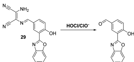
Scheme 27 A two-photon diaminomaleonitrile (DMN)-based ESIP fluorescent probe 29 for the selective detection of \text{HOCl}/\text{ClO}^- in RAW 264.7 cells and hippocampal brain slices. Measurement conditions: PBS/DMF (8 : 2) pH = 7.4.
