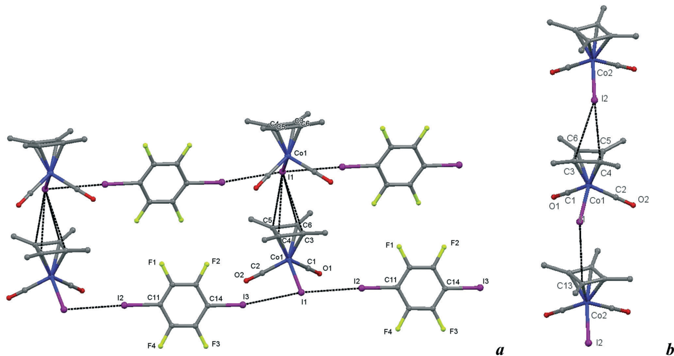
Fig. 8 a) Crystal structure diagram of 6 , showing a fragment of I-I halogen-bonded polymeric chains [\text{Cb}^*\text{Co}(\text{CO})_2\text{I}](\mu_2\text{-DITFB})_n linked by \text{I}-\pi(\eta_4\text{-Me}_4\text{C}_4) interactions. Hydrogen atoms are omitted for clarity. Selected distances (Å): intramolecular \text{Co}(1)-\text{I}(1) , 2.619(1); intermolecular \text{I}(3)-\text{I}(1) , 3.589(1); \text{I}(1)-\text{I}(2) , 3.585(1); \text{I}(1)-\text{C}(3-6) ring of the \eta^4 = \text{Me}_4\text{C}_4 ligand, 3.781(7)–3.866(7). Selected angles ( ^\circ ): \text{I}(3)-\text{I}(1)-\text{I}(2) , 171.51(2); \text{Co}(1)-\text{I}(1)-\text{I}(3) , 93.00(2); \text{Co}(1)-\text{I}(1)-\text{I}(2) , 95.16(2); \text{C}(14)-\text{I}(3)-\text{I}(1) , 169.6(2); \text{C}(11)-\text{I}(2)-\text{I}(1) , 177.2(2). b) Comparison of the \text{Cb}^*\text{Co}(\text{CO})_2 stacks in 6 with those in the parent crystal. Selected distances (Å): intermolecular \text{I}(2)-\text{C}(4) , 3.725(8); \text{I}(2)-\text{C}(3) , 3.87(1); \text{I}(1)-\text{C}(13) , 3.842(9), and similarities of the intramolecular distances \text{Co}(2)-\text{I}(2) , 2.598(1); \text{Co}(1)-\text{C}(2) , 1.781(7); \text{C}(2)-\text{O}(2) , 1.157(9); \text{Co}(1)-\text{C}(1) , 1.79(1); \text{C}(1)-\text{O}(1) , 1.16(1). Dotted lines link specific atoms at a distance shorter than the sum of their vdW radii. 18
