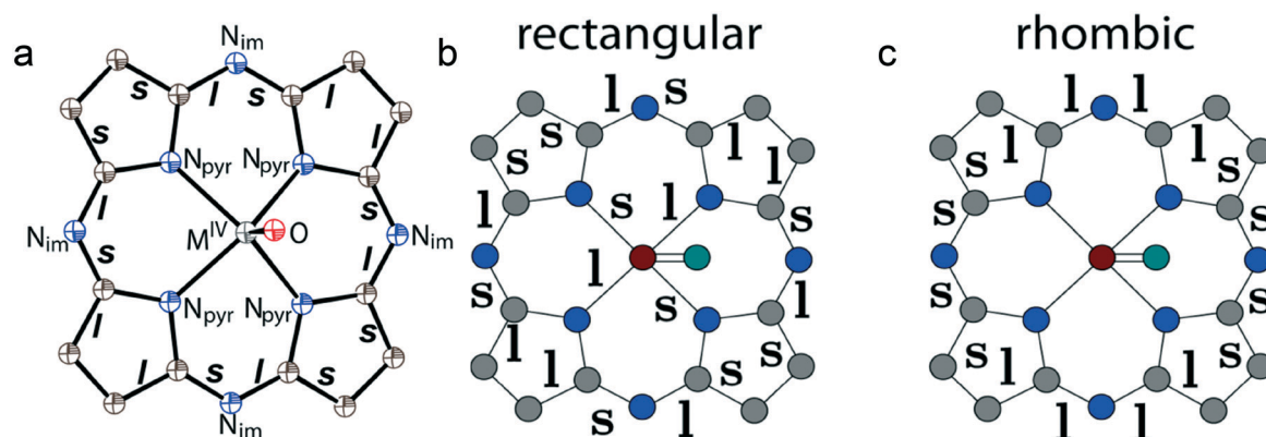
Fig. 13 (a) Experimentally observed alternation of the C–N(imine) and C–C pyrrole bonds in the {M IV O(Pc 3- ) ·- } radical anions. Schematic diagrams of the theoretically predicted rectangular (a global minimum) (b) and rhombic (a saddle point). (c) The C 2v JT deformations of the central part of the {M IV O(Pc 3- ) ·- } radical anions. The symbols l and s indicate C,N...C,N bonds which are elongated and shortened, respectively, at the reduction of Pc 2- to Pc 3- .
