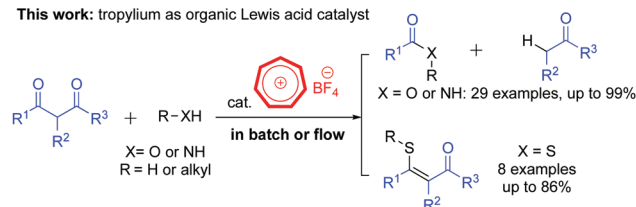
Scheme 1 retro -Claisen reactions.
