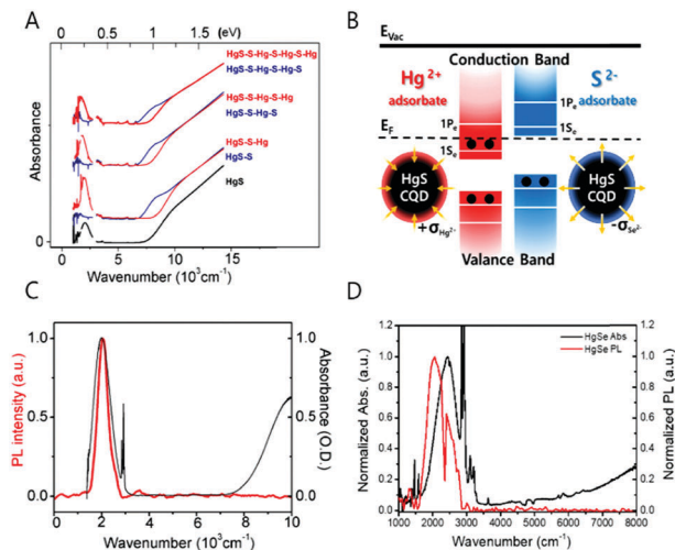
Fig. 4 (A) Absorption spectra of HgS CQD with S^{2-} and Hg^{2+} layer by layer growth. Reprinted with permission from ref. 36 copyright 2014 American Chemical Society. (B) Surface treatment schematics of HgS CQD (C) HgS absorption and photoluminescence spectra reprinted with permission from ref. 39. Copyright 2014 American Chemical Society. (D) HgSe absorption and photoluminescence.
