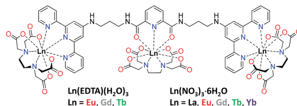
Fig. 1 Structural formula of multidentate tdt ligand composed of dpa and two tpy units free for binding Ln(EDTA)·(H 2 O) 3 or Ln(NO 3 ) 3 ·6H 2 O.
