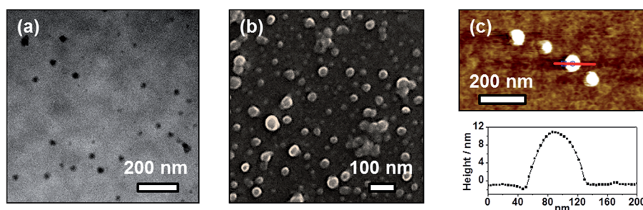
Fig. 6 (a) TEM and (b) SEM images prepared from a 300 \mu\text{M} solution of 1 in DMSO on carbon-coated copper grids. (c) Tapping mode AFM image of 1 showing aggregates on silica wafers; bottom: height profile observed along the red line shown.
