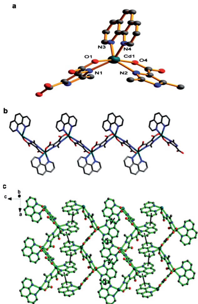
Fig. 15 (a) Molecular square structure of CP with [\text{Cd}(\text{HL})(\text{phen})]_n unit based on 2-ethyl-1 H -imidazole-4,5-dicarboxylic acid. (b) 1D chain of CP. (c) 2D sheet of CP supported by \pi - \pi stacking interactions. [Reprinted from ref. 158 Copyright 2012, with permission from Elsevier.]
