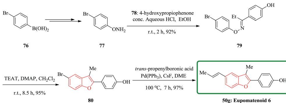
Scheme 17 Total synthesis of eupomatenoid 6 50g.
