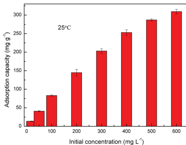
Fig. 6 The effect of initial concentrations (20, 50, 100, 200, 300, 400, 500, 600 mg\ L^{-1} ) on U(VI) removal by PAA hydrogels. (Volume, 10 mL; adsorbent dose, 0.01 g; pH value, 4.0; contact time, 180 min; temperature, 25 °C; rotating speed, 150 rpm.)
