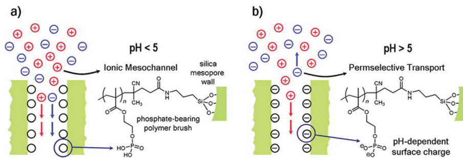
Fig. 22 Schematic depiction of the ionic transport processes taking place in the hybrid polymer–inorganic interfacial assembly at different pH values: (a) pH < 5, ionic mesochannel (no exclusion of ionic species) and (b) pH > 5, permeative transport of cations (Copyright 2012, The American Chemical Society, reprinted from ref. 247).
