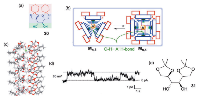
Fig. 6 (a) Structure of mannitol transporter 30 . (b) Schematic of how 30 self-assembles in lipid membrane. (c) Side-view of optimized structure of a 3 × 5 assembly of 30 containing a single Cl - anion. (d) Single-channel current traces recorded at 80 mV holding potential. (e) Inactive analogue 31 . The main conductance state is indicated by dotted lines. Reproduced from ref. 17. Copyright 2014, American Chemical Society.
