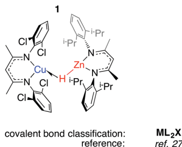
Fig. 3 A \sigma -zincane complex of \text{Cu}^I .
