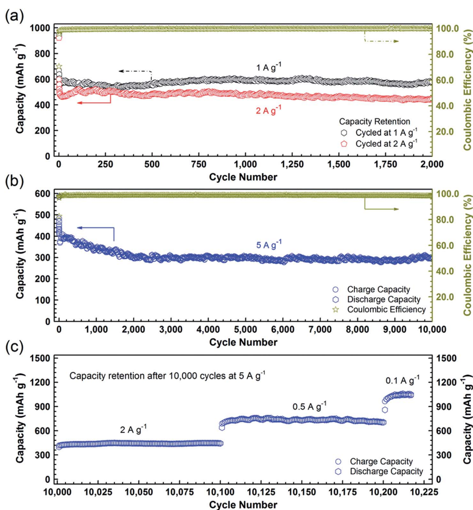
Fig. 5 Discharge/charge capacity and coulombic efficiency versus cycle number for the PCC-CoO x electrodes. (a) At current densities of 1 and 2 A g -1 for 2000 cycles. (b) At a current density of 5 A g -1 for 10 000 cycles after aging for five cycles at 0.1 A g -1 . (c) Subsequent capacity retention at various current densities from 2 to 0.1 A g -1 after 10 000 cycles at 5 A g -1 .
